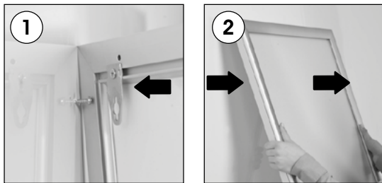
Hanger mounting
