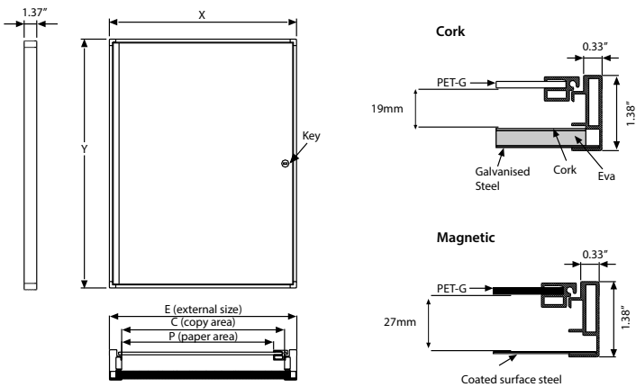
Size of boards for all Officeboard models:
