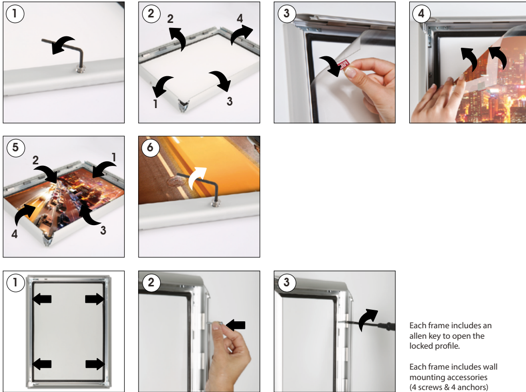
Screw & anchor mounting
