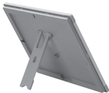
The opened position of counter support for Opti Frame in horizontal position.
